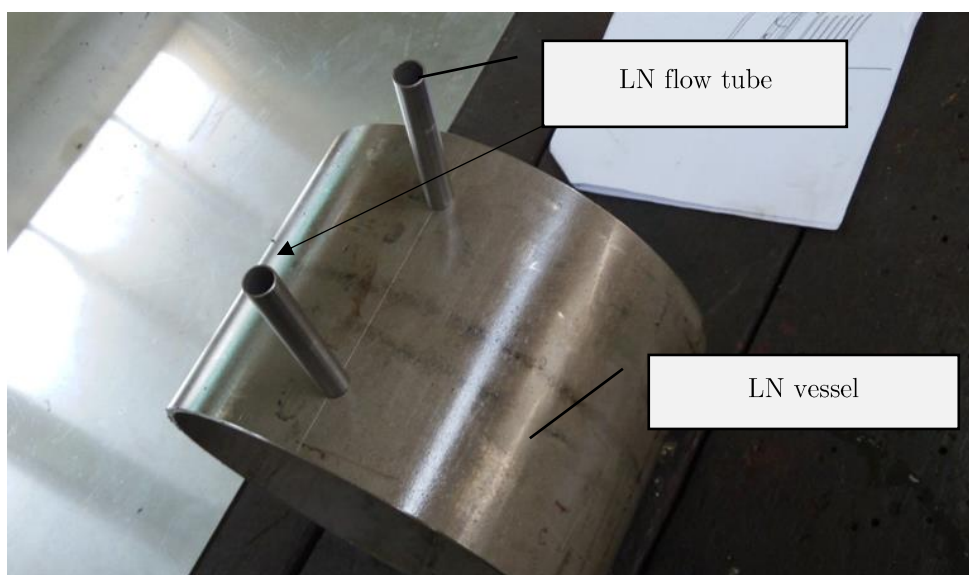
Figure 2: Simple Continuous Flow (SCF) Cryostat Vessel and Tubing
