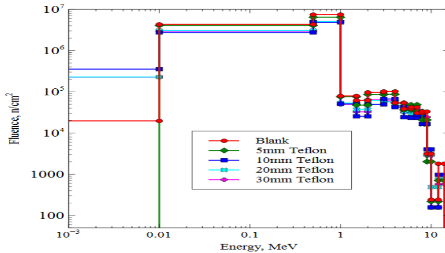
Figure 12: Neutron spectrum for Teflon with different thickness between room temperature and about -55^{\circ}C (MSpec-2).
