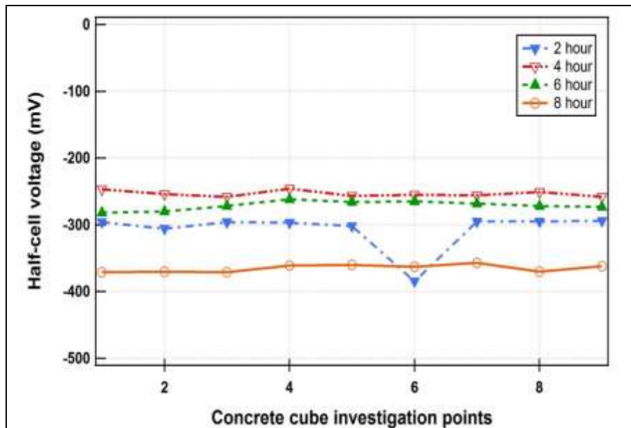
Figure 14. Half-cell voltage measurement on concrete cube investigation points for tap water analysis with different hours under the exposure of DC current.
