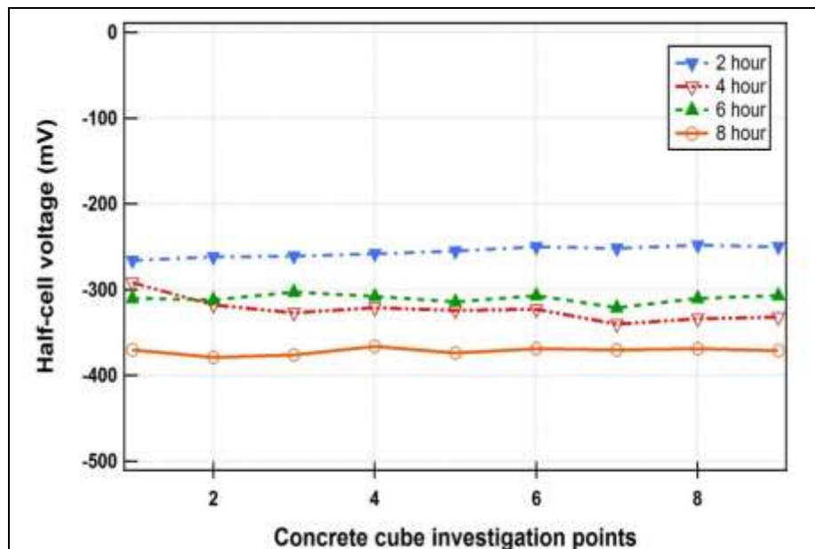
Figure 13. Half-cell voltage measurement on concrete cube investigation points for river water analysis with different hours under the exposure of DC current.
