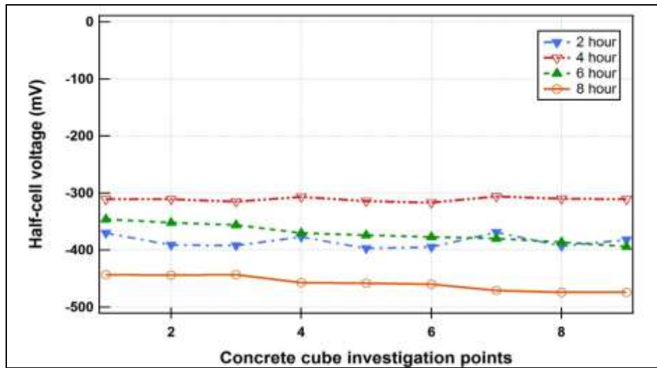
Figure 11. Half-cell voltage measurement on concrete cube investigation points for sea water analysis with different hours under the exposure of DC current.
