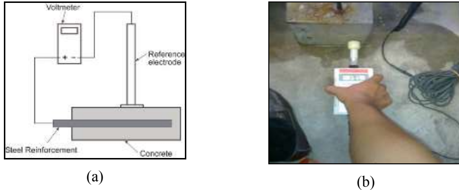
Figure 9. (a) Schematic diagram of half-cell potential measurement technique [7] and (b) Actual half-cell potential measurement using the reference electrode
