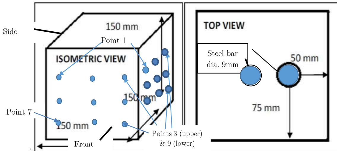
Figure 7. Concrete cube dimensions for testing purposes; points of half-cell probe measurement are indicated
