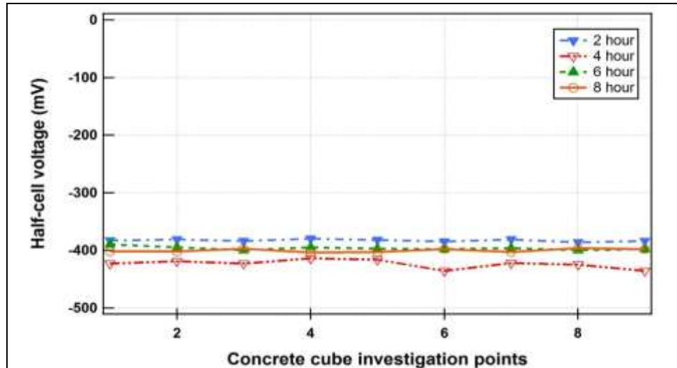
Figure 12. Half-cell voltage measurement on concrete cube investigation points for salt marsh water analysis with different hours under the exposure of DC current.
