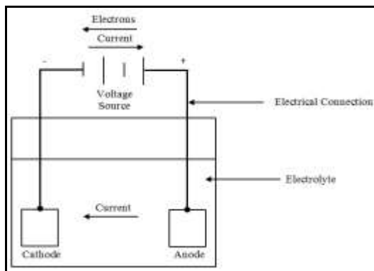
Figure 1. Schematic of a corrosion cell
