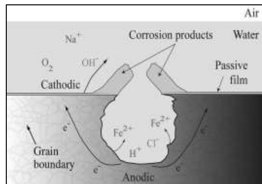
Figure 2. Corrosion processes on the steel surface (Fontana M.G., 1986)
